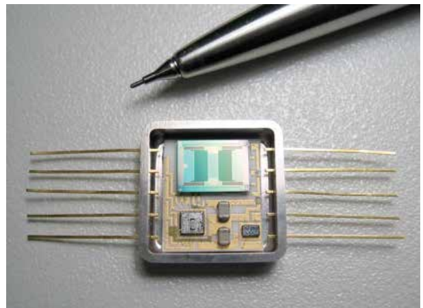
An example of a MEMS accelerometer. This is a large sensor typically used for inertial navigation (low frequency, high-precision applications). Although this device is much larger than the ecoCMS MEMS sensor, the underlying technology is similar, and the silicon wafer can be seen at the top of the enclosure. (Courtesy: ONYX InSight)
